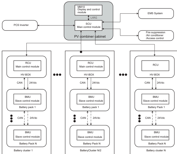
Architecture diagram of large storage system
